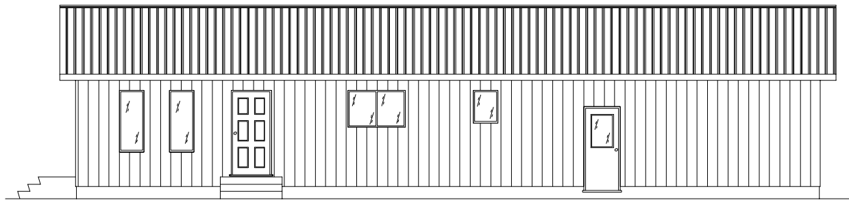
FRONT ELEVATION
